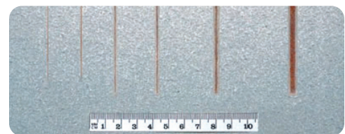
Fig. 2: Cut Edge Performance of GI & ZINCALUME® steel
