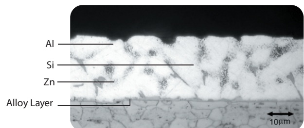
Fig. 1: Microstructure Cross Section of ZINCALUME® steel
