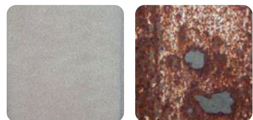
Fig. 3: Outdoor Exposure Performance - 21 years of exposure at severe marine test site.
